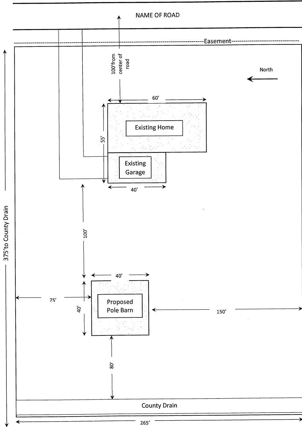
EXAMPLE OF PLOT PLAN:
